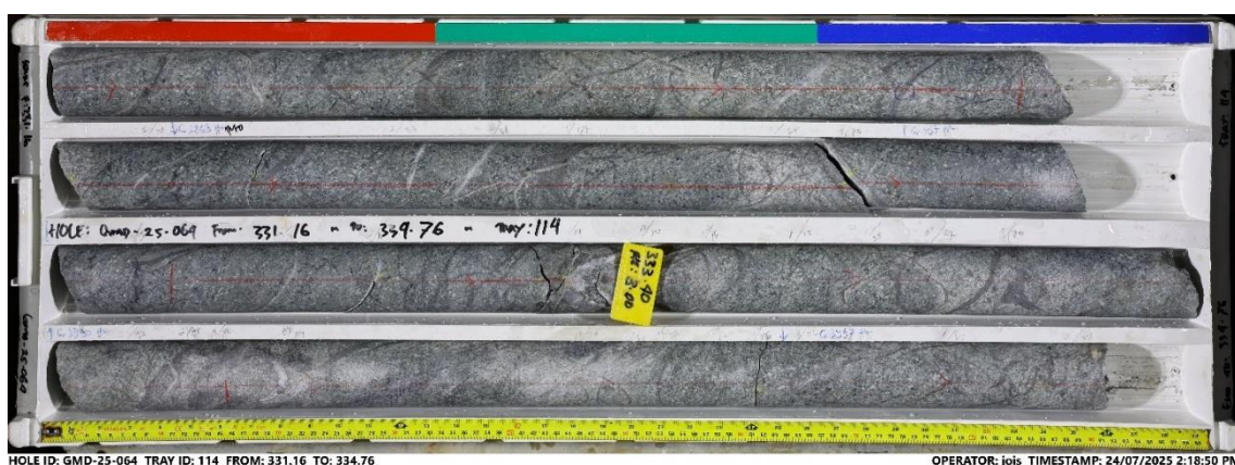
Figure 6: Gua Macan drill core from GMD-25-064 showing porphyry style stockwork quartz-magnetite-chalcopyrite veins.
