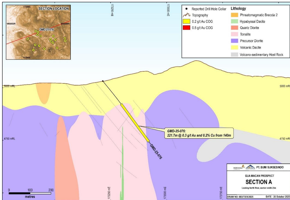
Figure 3: Gua Macan drill section A showing GMD-25-076, with mineralised intercepts
