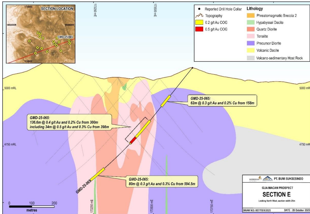
Figure 11: Gua Macan drill section E showing GMD-25-065 with mineralised intercepts
