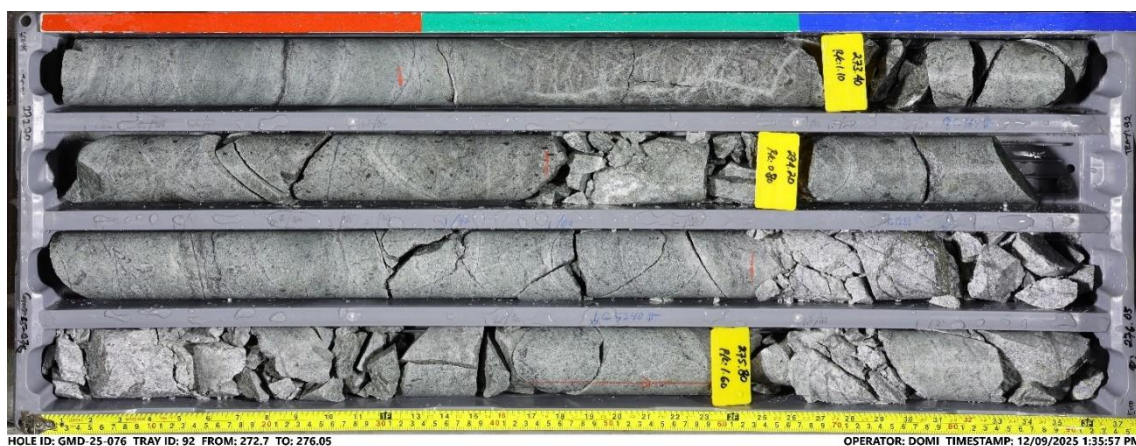
Figure 4: Gua Macan drill core from GMD-25-076 showing porphyry style stockwork quartz-magnetite-chalcopyrite veins.
