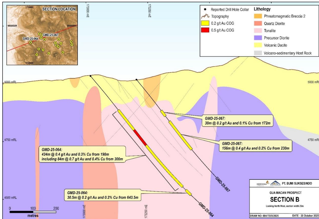
Figure 5: Gua Macan drill section B showing GMD-25-064 and GMD-25-067, with mineralised intercepts
