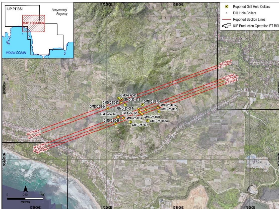
Figure 2: Plan view of Gua Macan drill sections and drill collars
