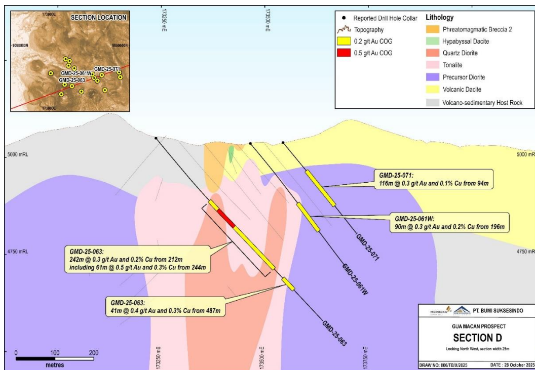
Figure 9: Gua Macan drill section D showing GMD-25-063, GMD-25-061W and GMD-25-071, with mineralised intercept
