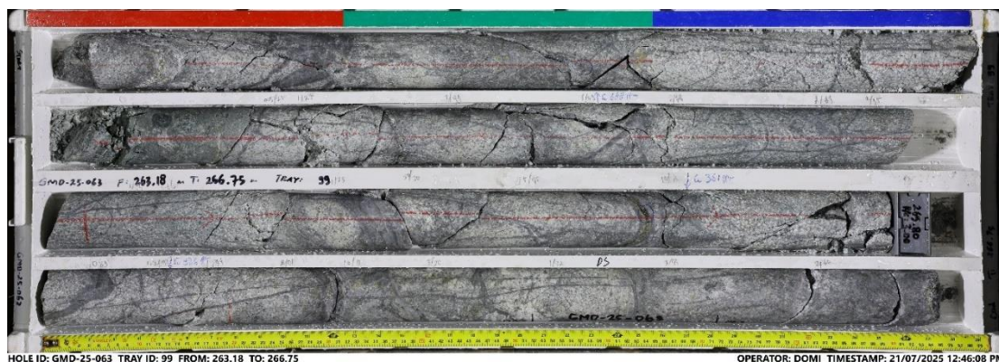
Figure 10: Gua Macan drill core from GMD-25-063 showing porphyry style stockwork quartz-magnetite-chalcopyrite veins.
