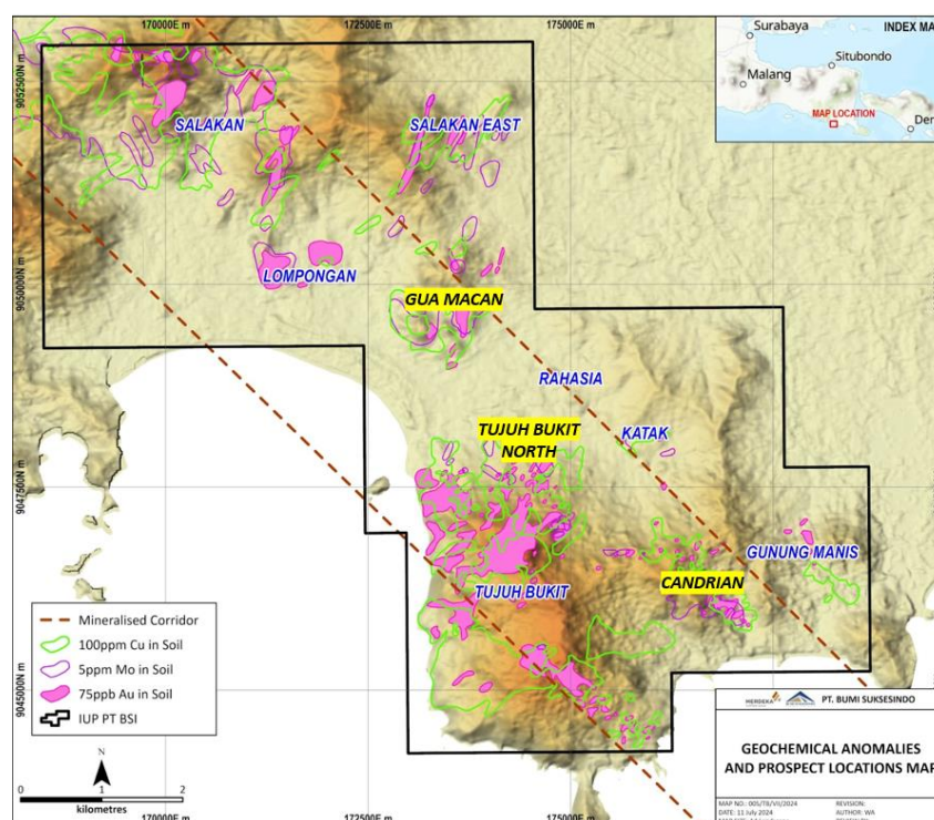
Figure 1: Tujuh Bukit Geochemical Anomalies and Prospect Locations
