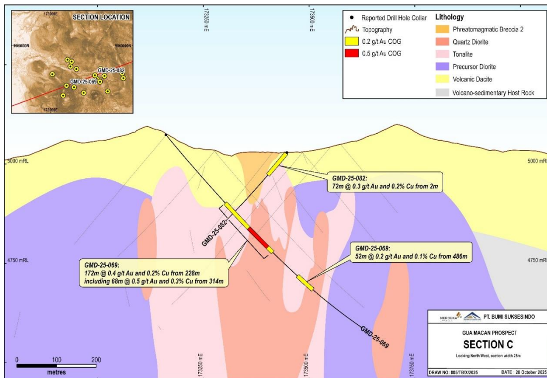
Figure 7: Gua Macan drill section C showing GMD-25-069 and GMD-25-082, with mineralised intercepts
