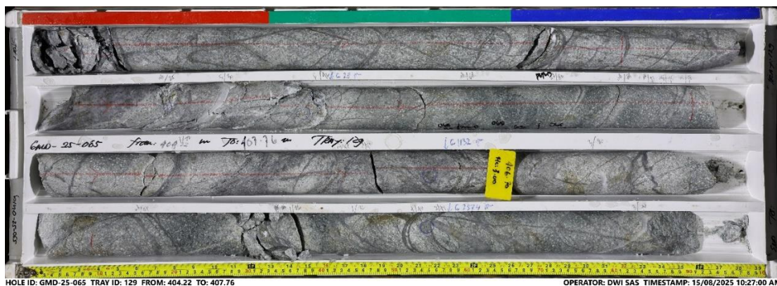
Figure 12: Gua Macan drill core from GMD-25-065 showing porphyry style stockwork quartz-magnetite-chalcopyrite veins.
