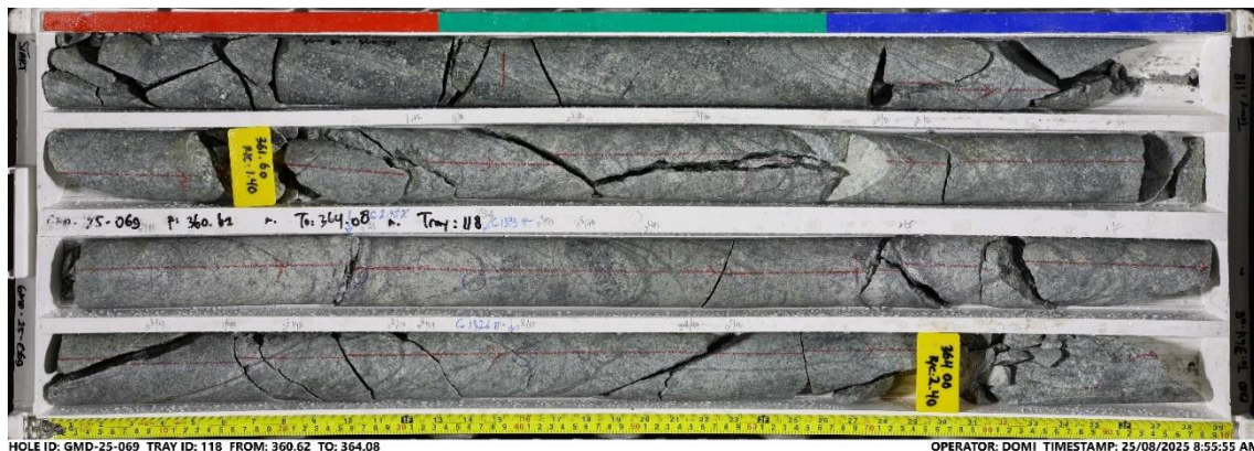
Figure 8: Gua Macan drill core from GMD-25-069 showing porphyry style stockwork quartz-magnetite-chalcopyrite veins
